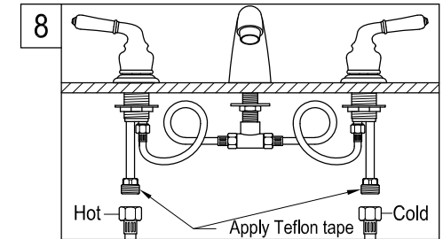
Teflon Tape
